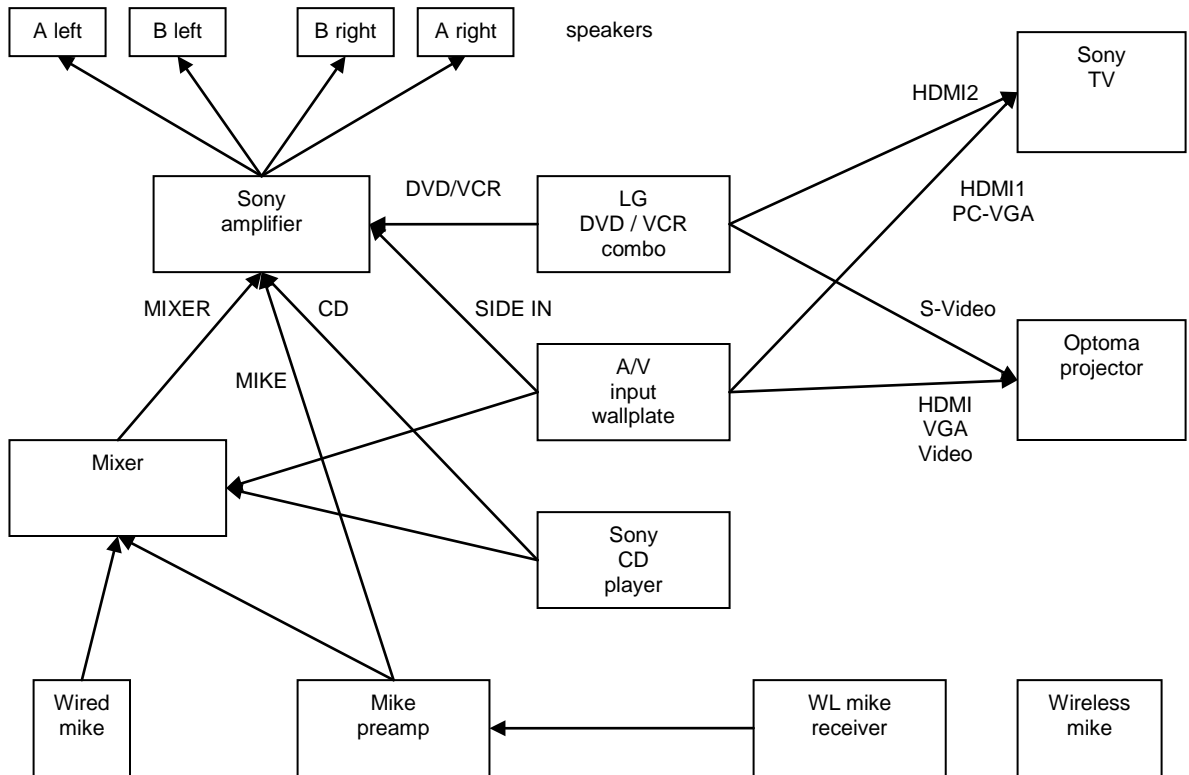
Figure 2. A/V box functional connections
